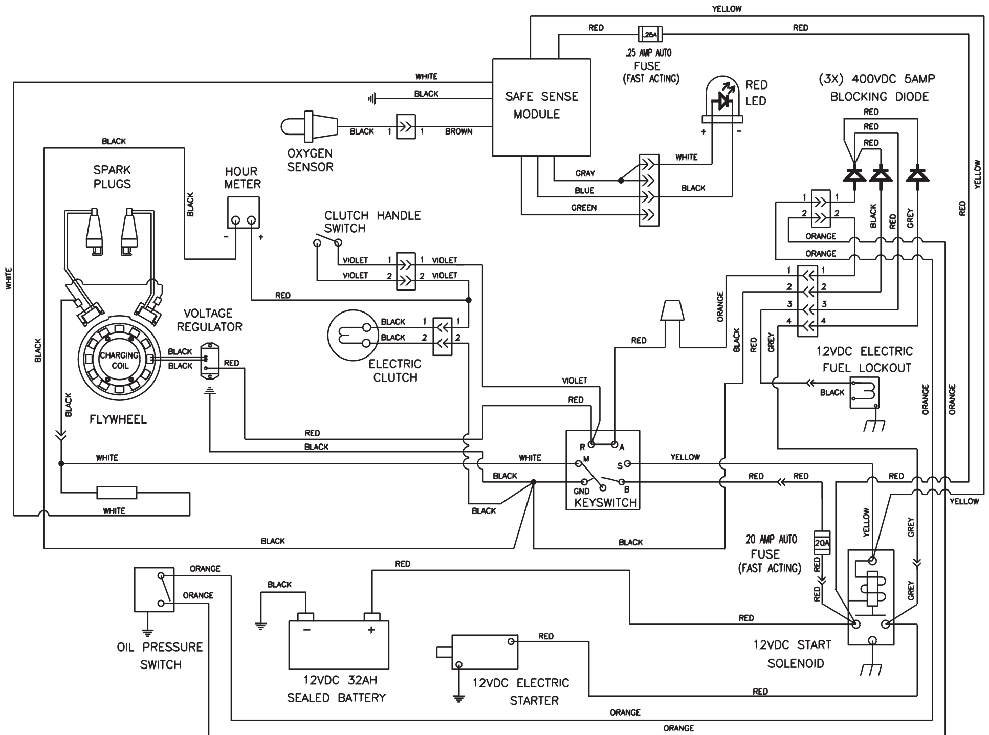
ELECTRICAL SCHEMATIC SAFE SENSE
